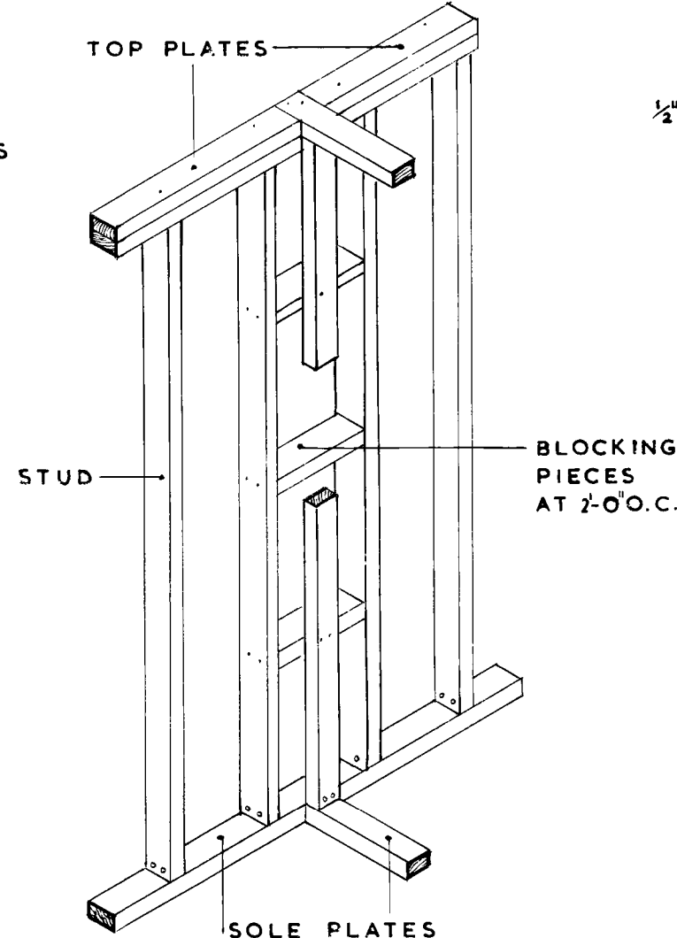
FRAMING FOR LIVING ROOM WINDOWS
