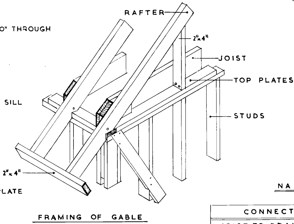
FRAMING OF GABLE
