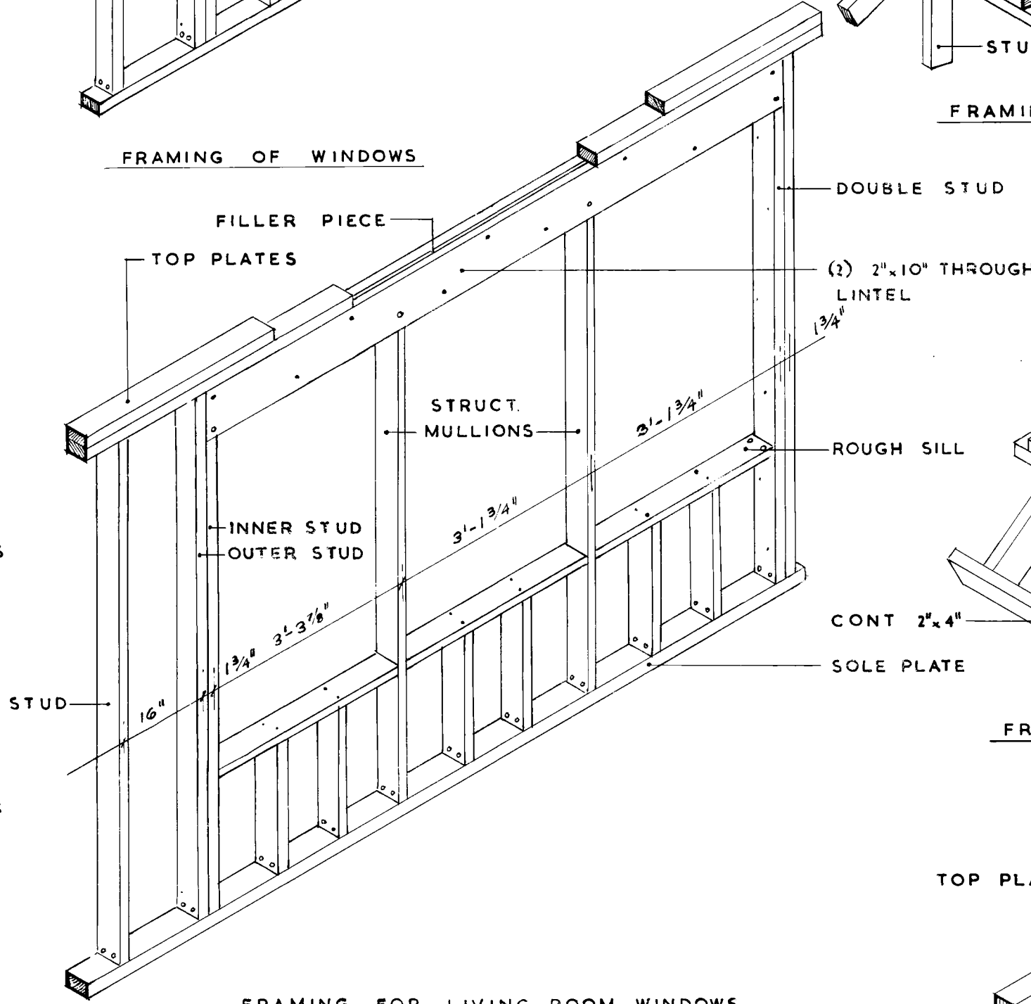
FRAMING FOR LIVING ROOM WINDOWS
