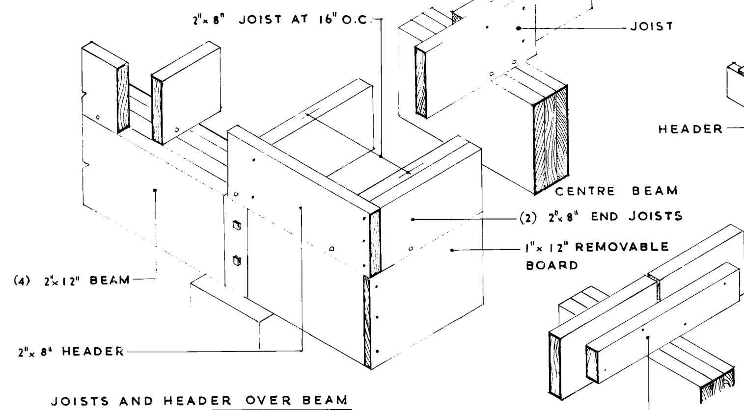
JOISTS AND HEADER OVER BEAM
