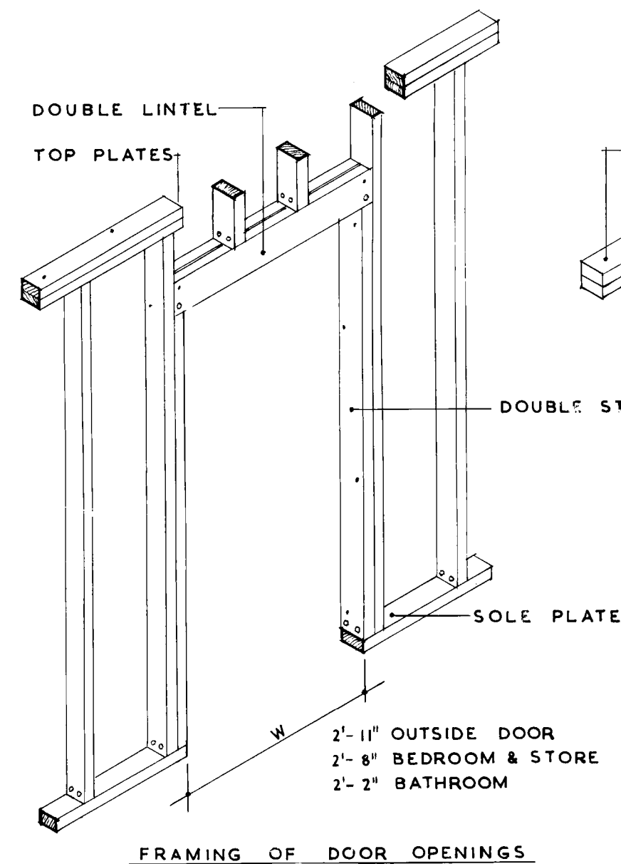
FRAMING OF DOOR OPENINGS
