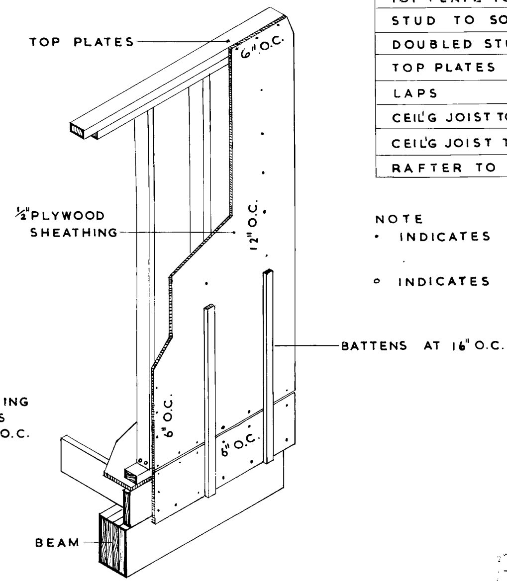
NAILING OF WALL SHEATHING
