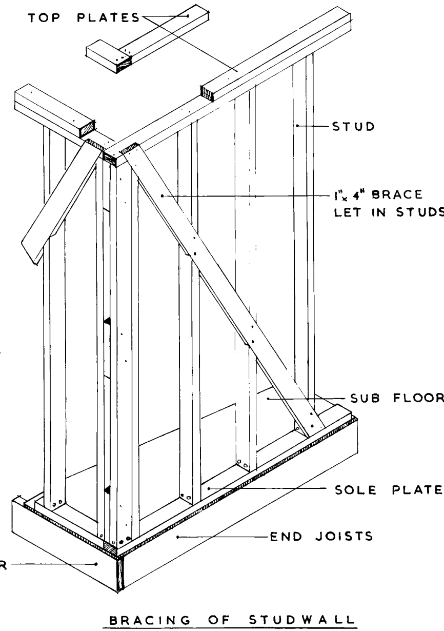
BRACING OF STUD WALL
