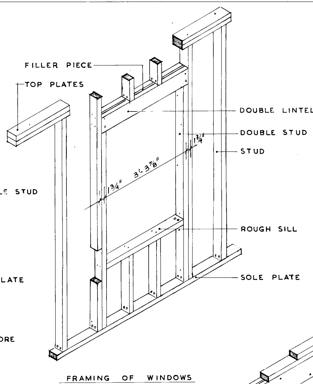
FRAMING OF WINDOWS
