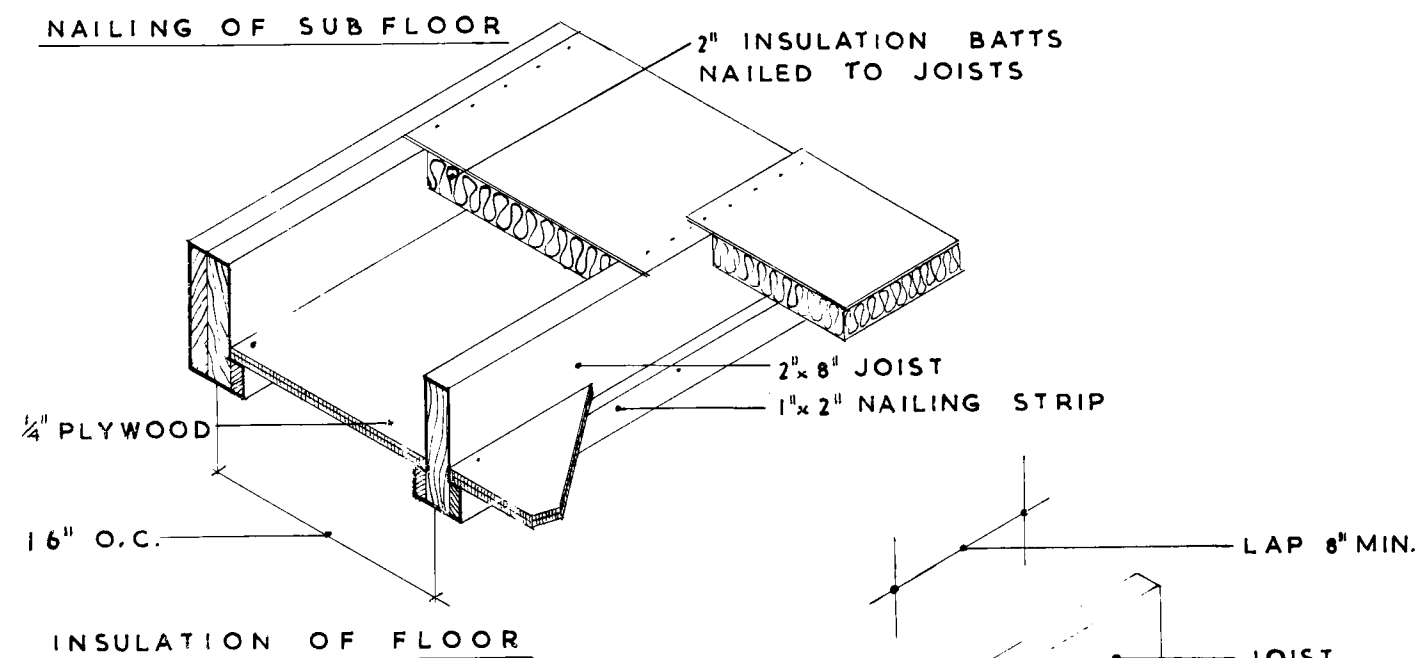
INSULATION OF FLOOR
